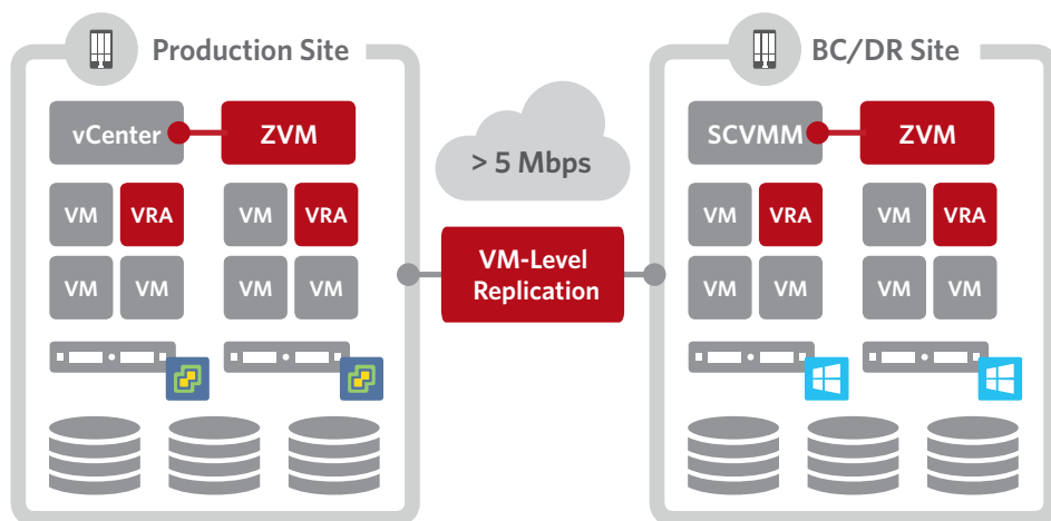
Figure 5. Zerto's Architecture
